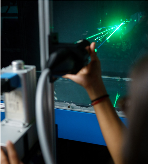
Student researcher setting up laser doppler velocimeter for inflow velocity measurement in low-Reynolds-number aerodynamics experiment.
